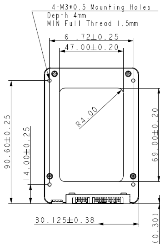
(Bottom View)
