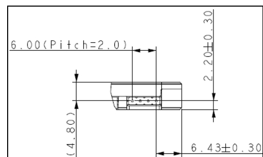
(Pin Detail)
